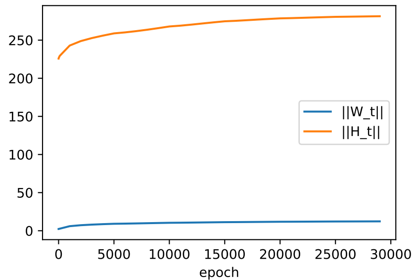
Norm
